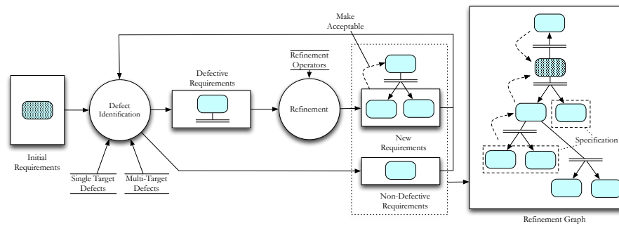
Fig. 4 Overview of the Approach
