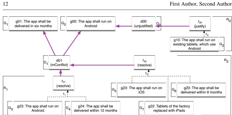
Fig. 5 Example of Construction of ASPIC + Arguments
