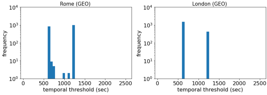
Fig. 8 Time threshold distributions for the users obtained by ACTS_{LOC} in Rome and London. Compared to ATS , the distributions are more concentrated on the two peaks.
