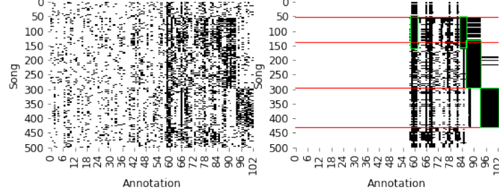
Fig.1: CAL500 Music dataset. The left side shows the bitmap of the binary annotation matrix where objects represent songs and attributes represent annotations (black=presence; white=absence). The right side shows the bitmap of the identified co-clusters. Objects and attributes are ordered in the same way in both figures just for visualization purpose. (best seen in color)
