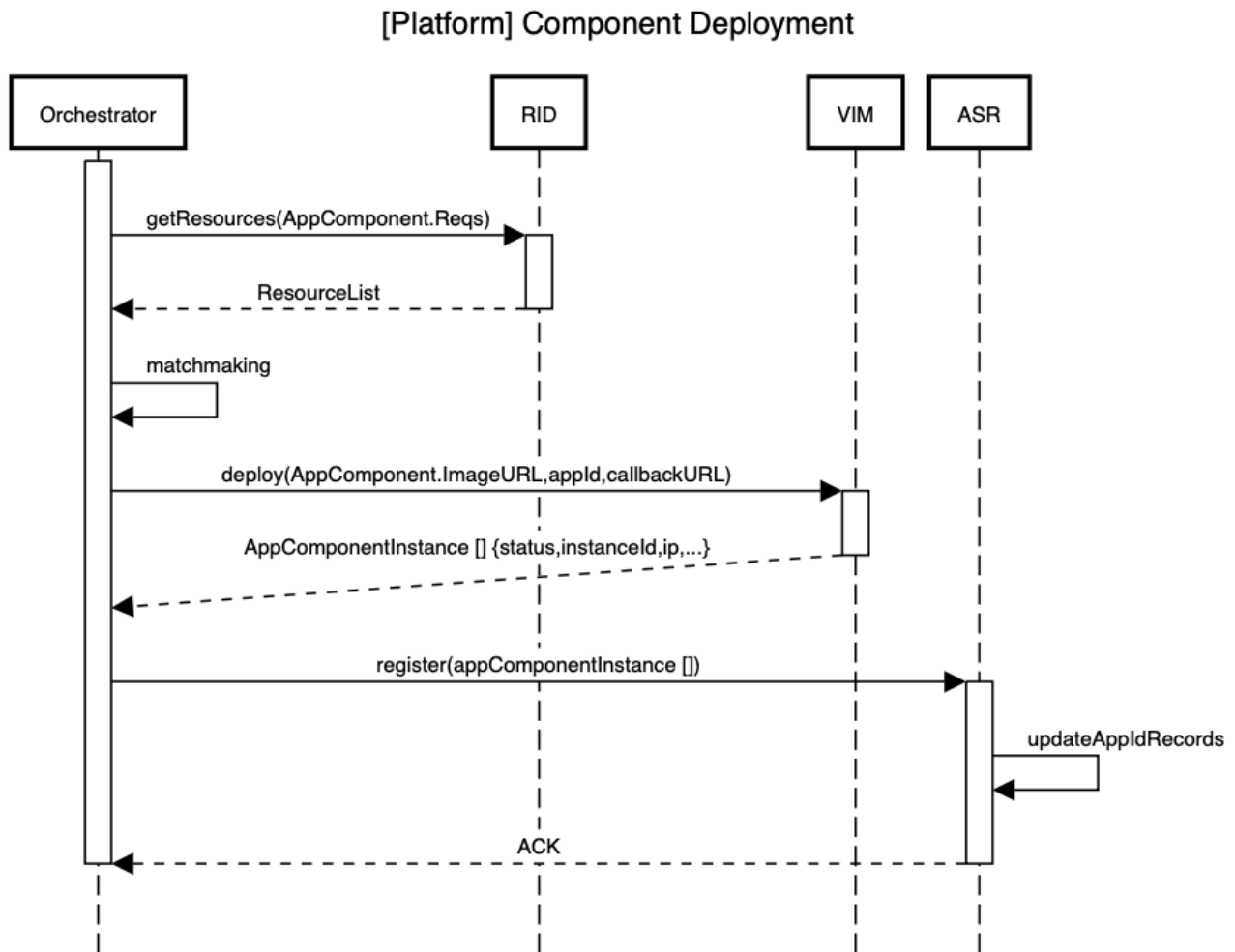
Figure 3-1: Platform Component Deployment
