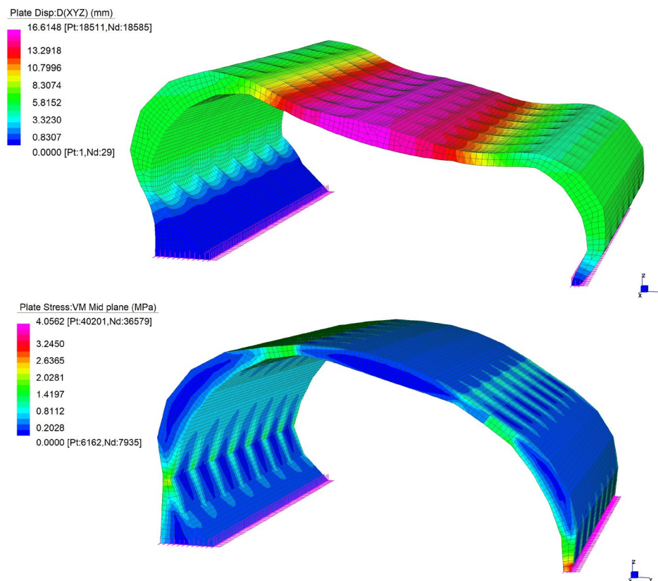
Figure 7: Case study results: top, magnified 15% SLS displacement; bottom, von Mises stress at ULS
