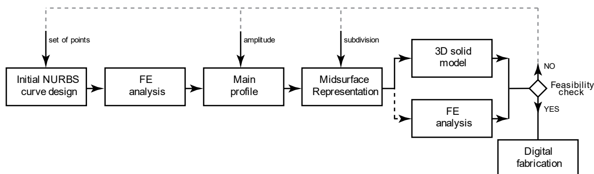
Figure 2: Flow chart adopted in the design and verification of the recycled-HDPE pavilion
