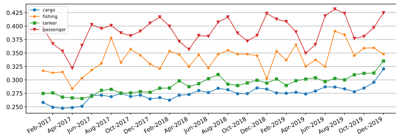
Figure 5: Fraction of bidirectional edges
