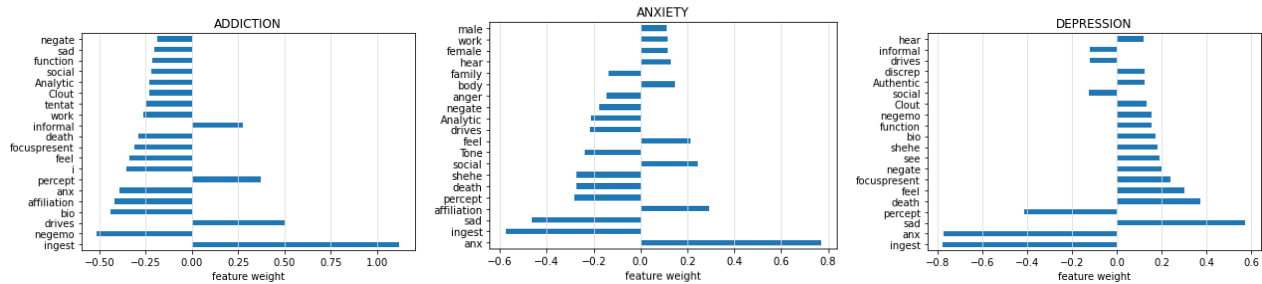
Figure 8: The most important features of SVM model. Each plot represents the 20 highest coefficients of the hyperplane dividing data points of a certain category from the others.
