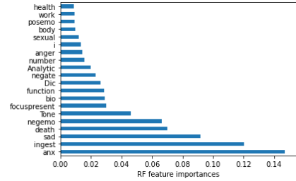
Figure 7: The 20 most important features of the psychometric profile for RF
