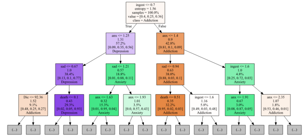
Figure 6: Split nodes of the first levels of the Decision Tree
