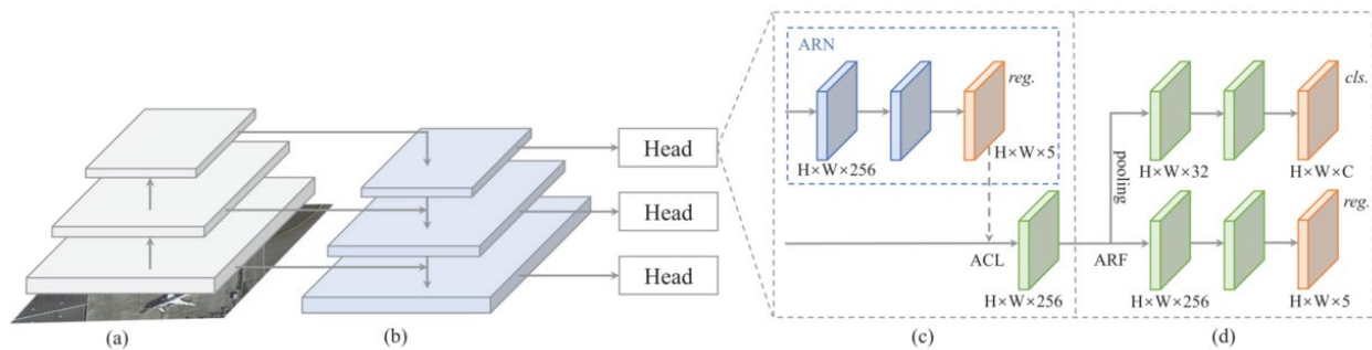
Figura 2-9: Architettura di S²A Net (single-shot alignment network) (Han, 2021).
