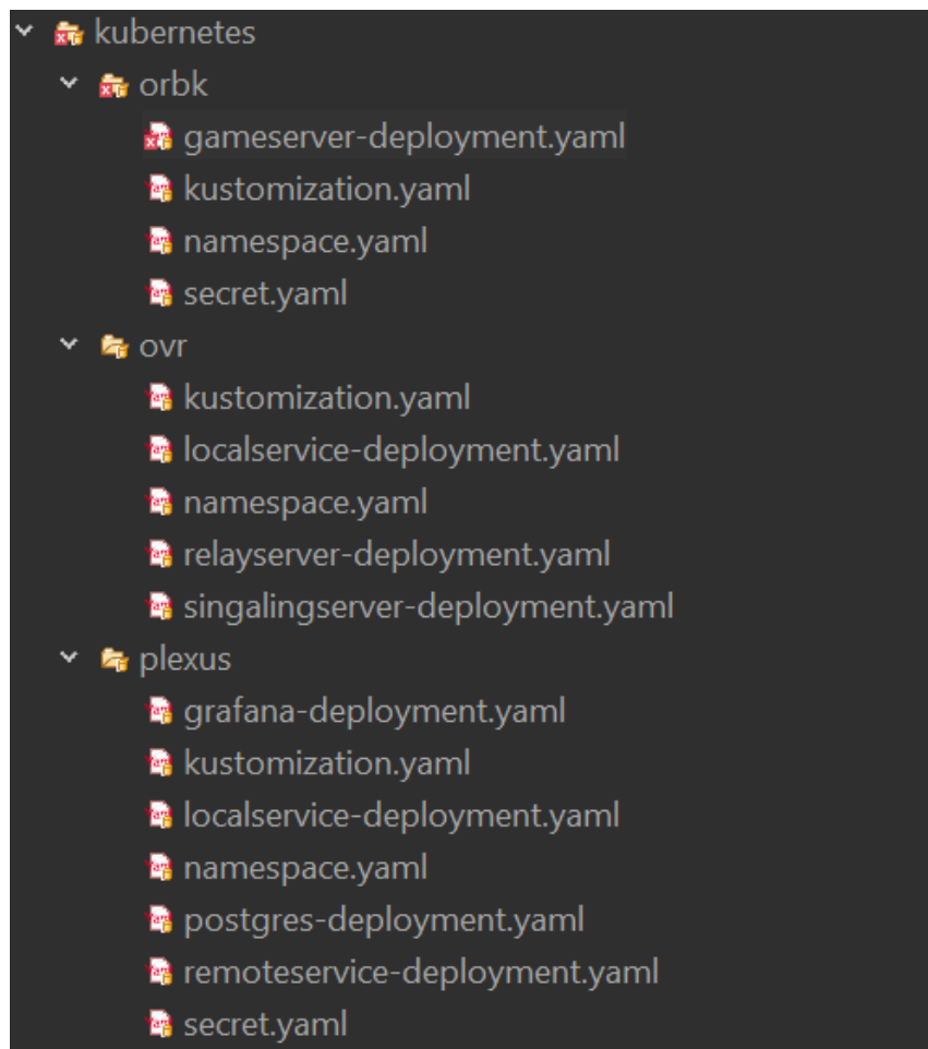
Figure 3: K3s Yaml files produced by the Converter component for each Use Case
