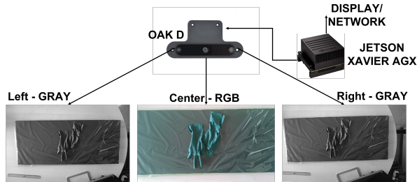
Fig. 2. Overview of the acquisition using OAK-D camera [17].
