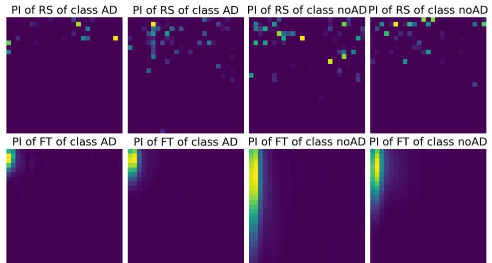
Figure 1. First row: Two persistence images (PI) of the spectra for class AD and two for class noAD. Second row: two PI of the FT for class AD and for class noAD.
