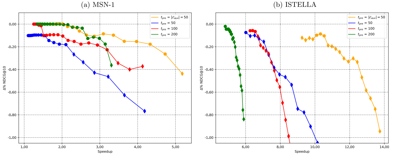
FIGURE 2. Estimated impacts on the validation set of different sentinel positions for EPT on MSN-1 and ISTELLA. Points are marked with a circle if there is statistical equivalence between the NDCG values of the EE solution and those from the baseline and with a diamond otherwise.
