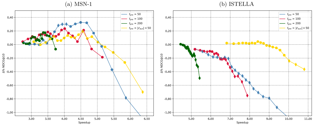
FIGURE 3. Estimated impacts on the validation set of different sentinel positions for LEAR on MSN-1 and ISTELLA. Points are marked with a circle if there is statistical equivalence between the NDCG values of the EE solution and those from the baseline and with a diamond otherwise.
